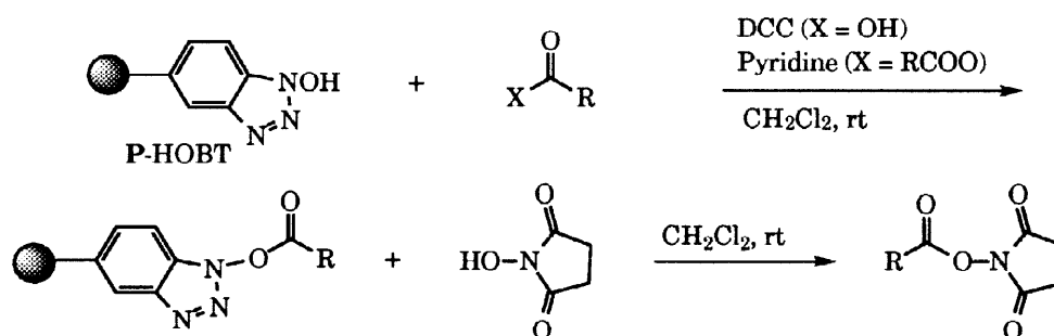
Scheme 1. General method for NHS ester synthesis
